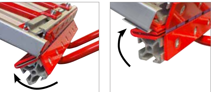
Step 1: Bevelling to approx. 170 degrees
