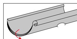
Prepare the gutter / Flange the gutter hole
