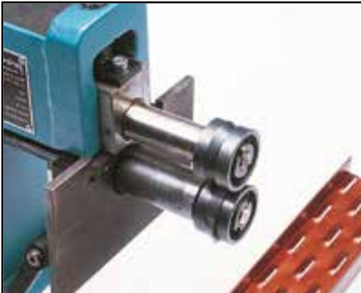
MASC Longitudinal slot rolls enable uniform and equally deep cut-outs without time-consuming measuring and marking.
