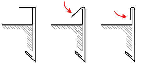
Front board panelling by changing rollers in 2 work steps (for wider edgings)
