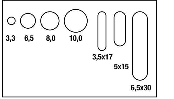
Stamps & dies
